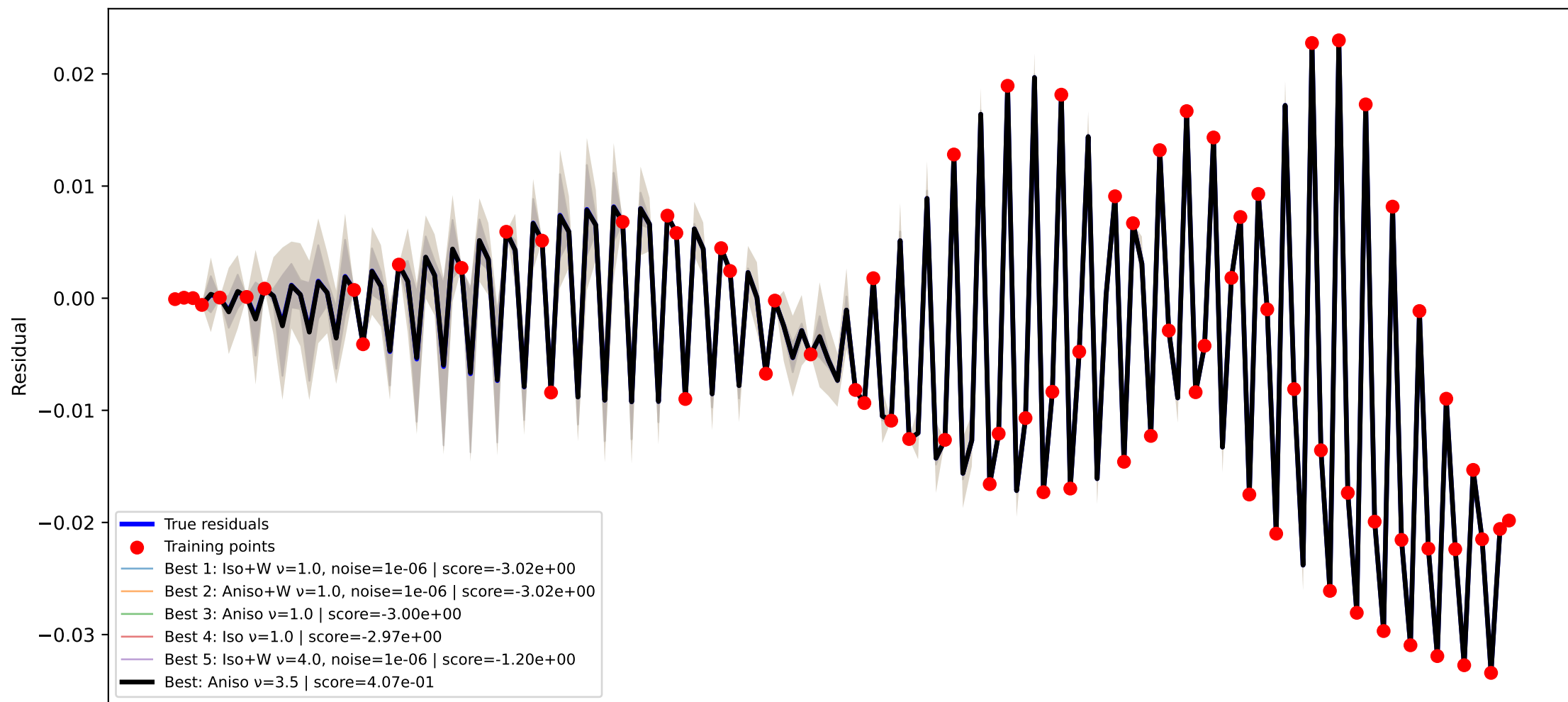
GPR kernel comparison node=48 RMSE=3.903e-05, train RMSE=5.185e-11
